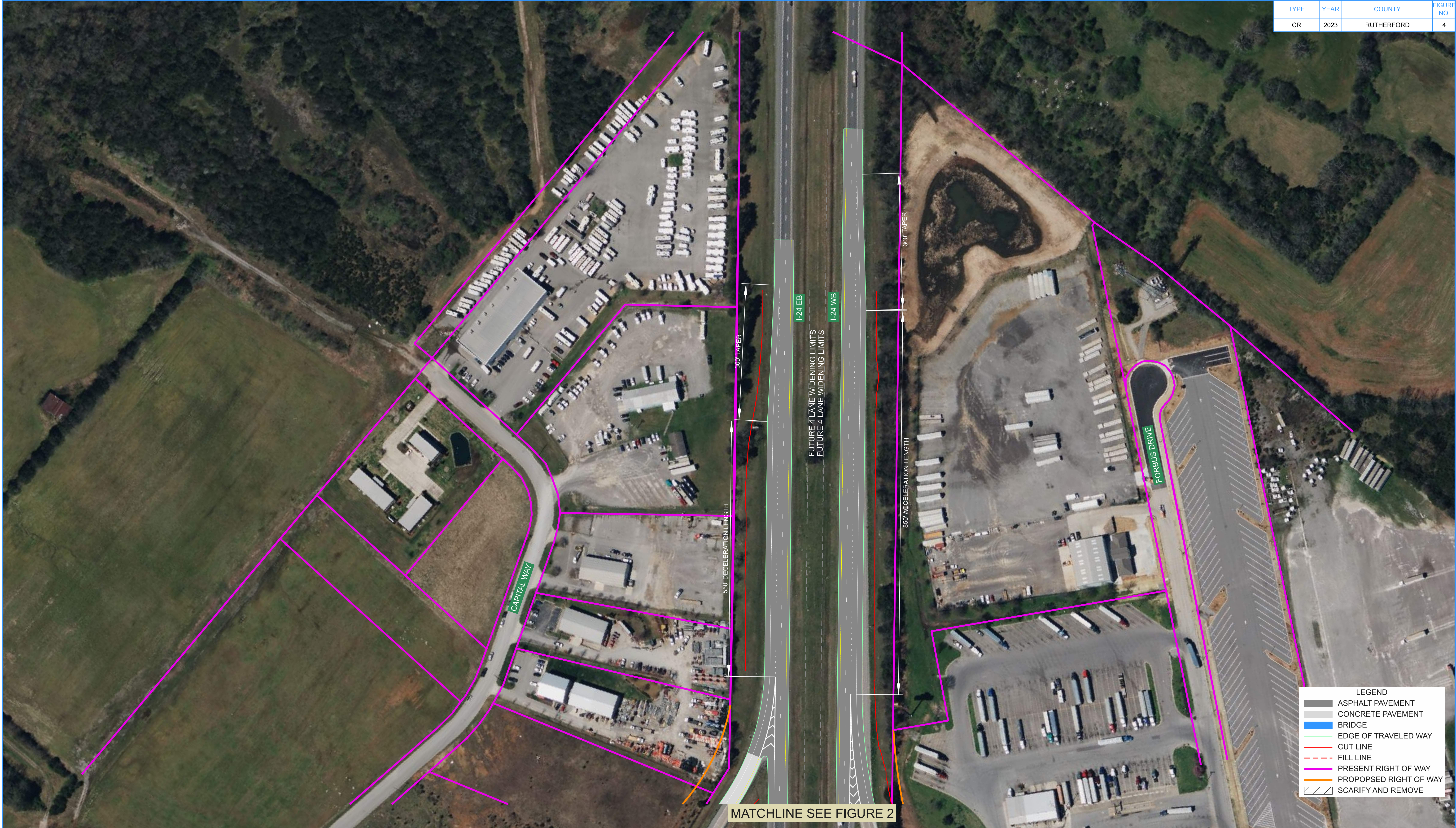
FIGURE 4 I-24 INTERCHANGE AT EPPS MILL ROAD (EXIT 89) CONCEPTUAL PLAN
