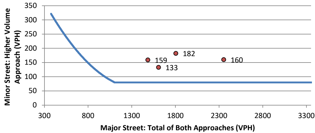
Warrant 2: Four-Hour Vehicular Volume
