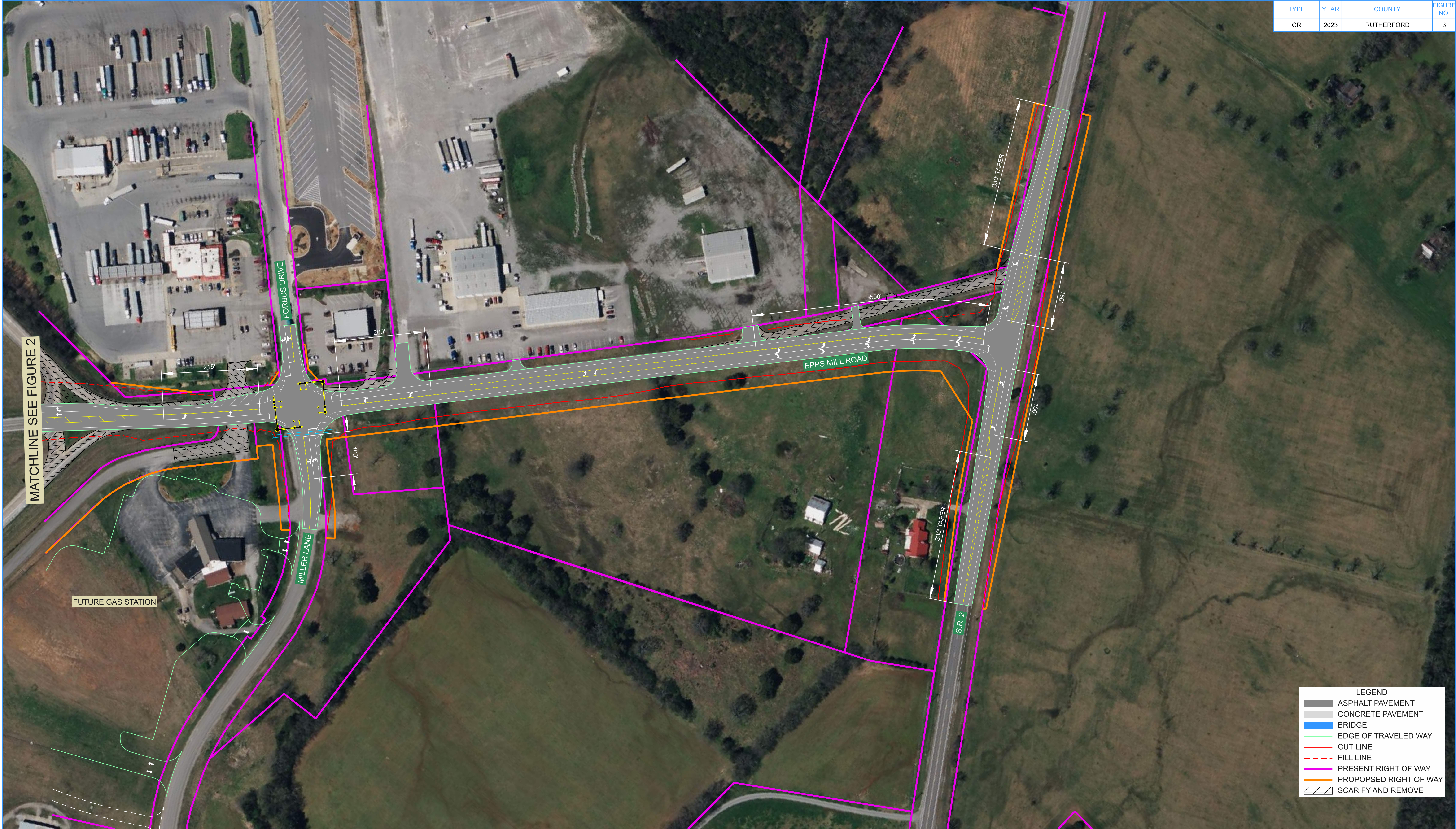
FIGURE 3 I-24 INTERCHANGE AT EPPS MILL ROAD (EXIT 89) CONCEPTUAL PLAN
