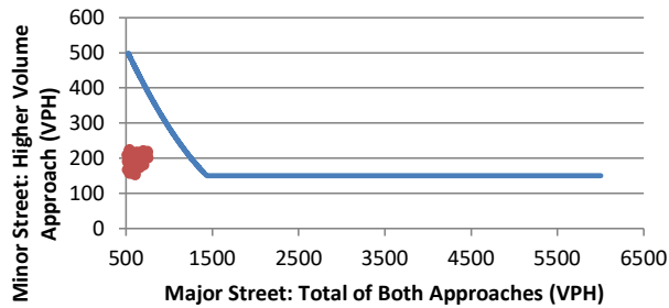
Warrant 3: Peak Hour
