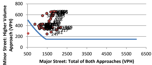
Warrant 3: Peak Hour
