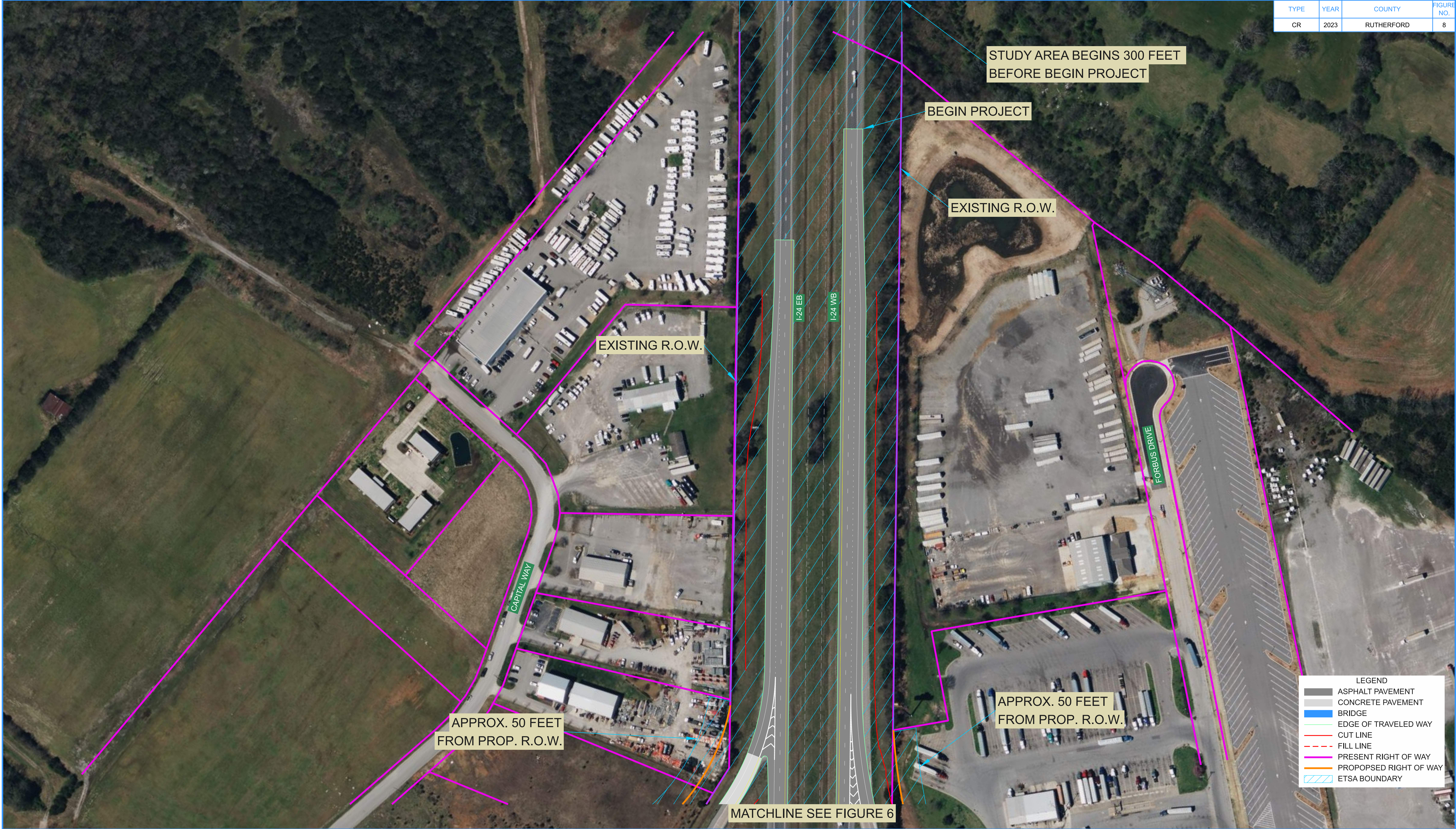
FIGURE 8 I-24 INTERCHANGE AT EPPS MILL ROAD (EXIT 89) ETSA
