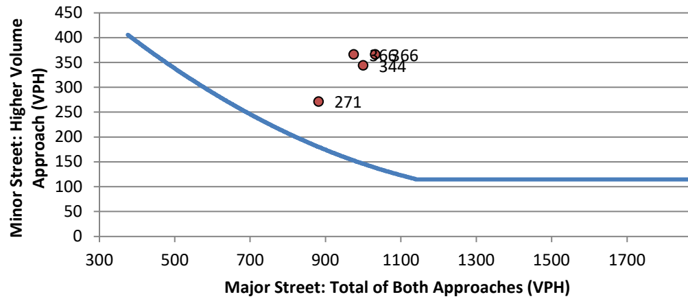
Warrant 2: Four-Hour Vehicular Volume
