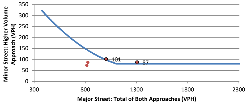
Warrant 2: Four-Hour Vehicular Volume
