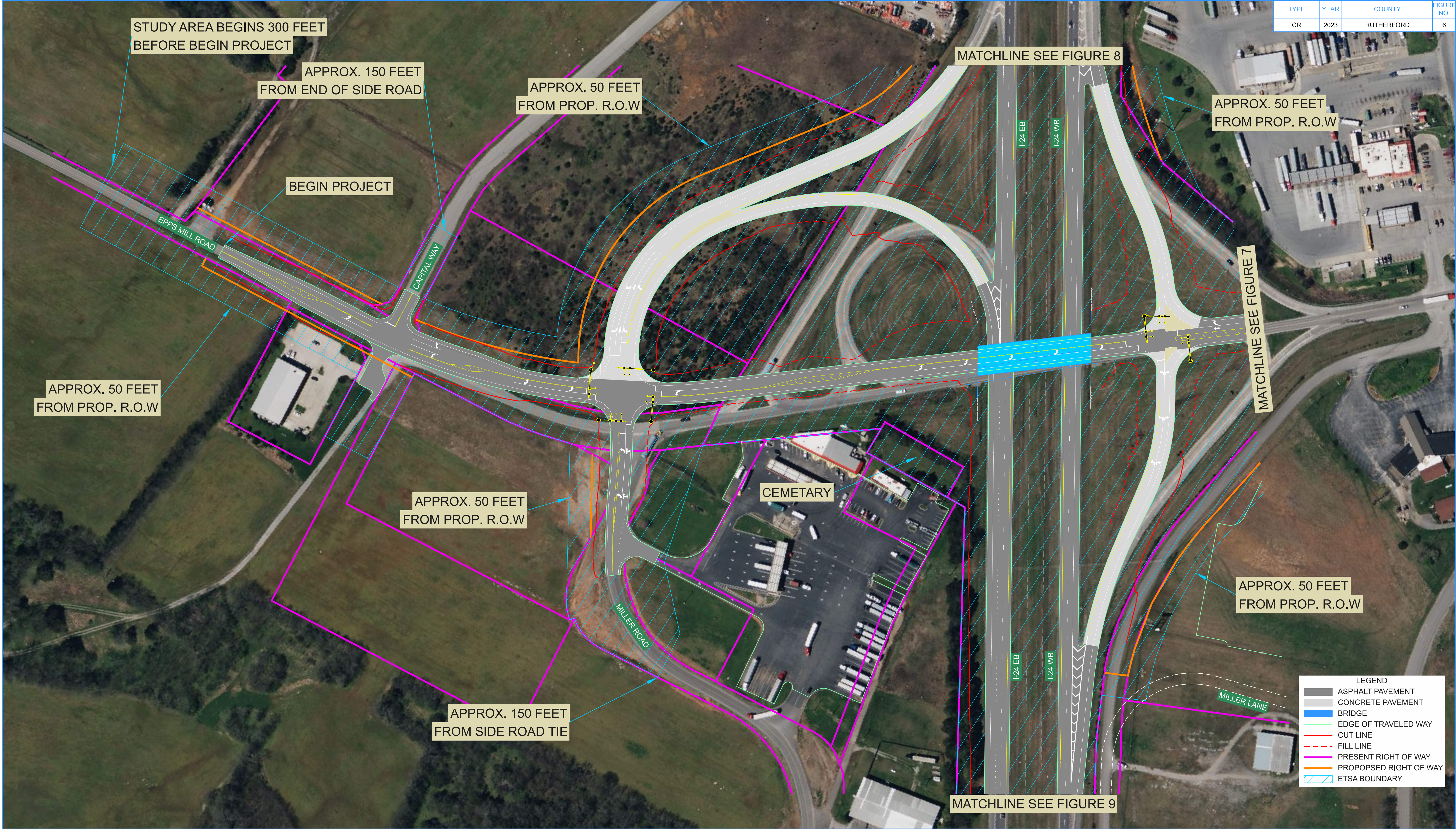
FIGURE 6 I-24 INTERCHANGE AT EPPS MILL ROAD (EXIT 89) ETSA
