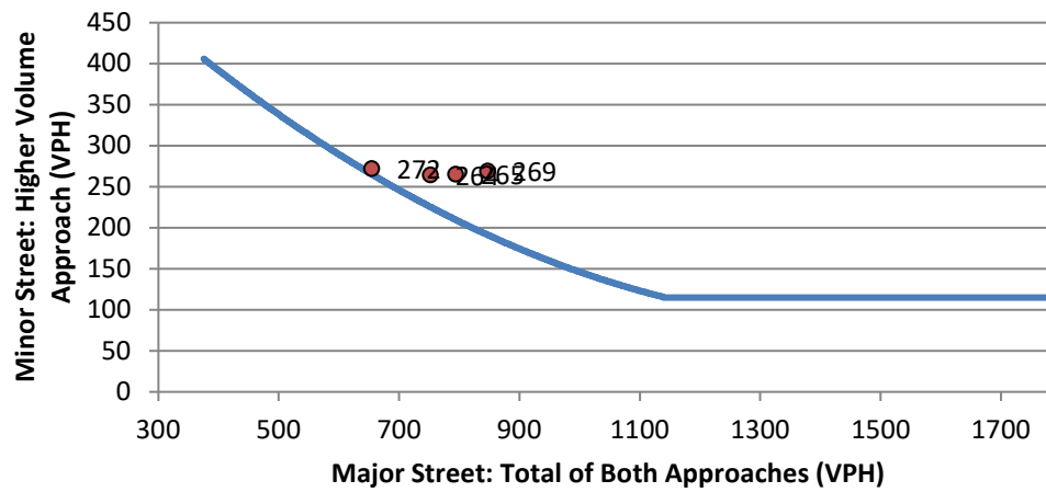
Warrant 2: Four-Hour Vehicular Volume
